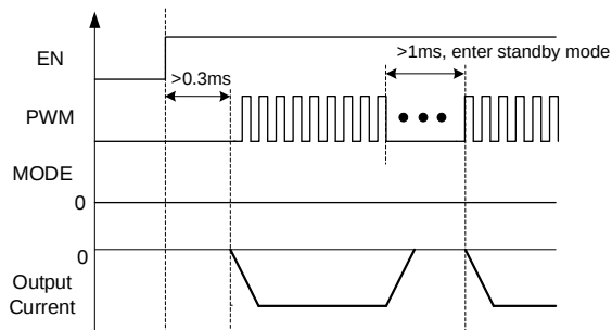
Figure 3: Negative Output Current Mode
