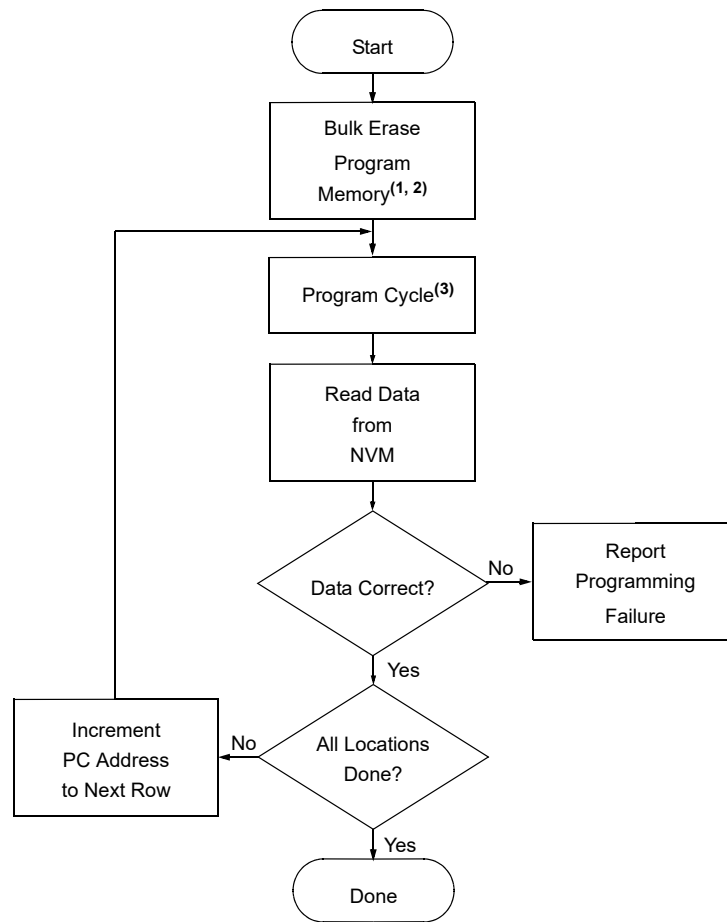
Figure 3-17. Program Memory Flowchart
