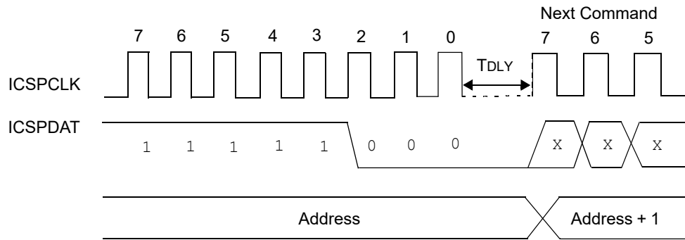
Figure 3-12. Increment Address
