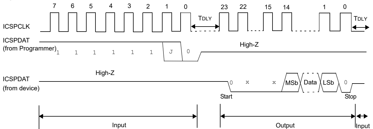
Figure 3-11. Read Data from NVM
