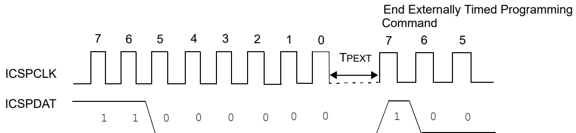
Figure 3-14. Begin Externally Timed Programming
