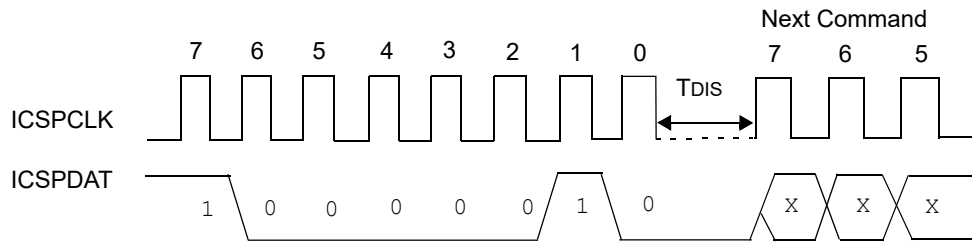
Figure 3-15. End Externally Timed Programming
