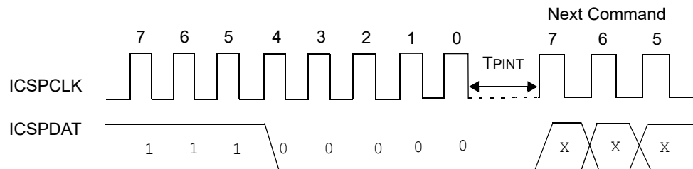
Figure 3-13. Begin Internally Timed Programming
